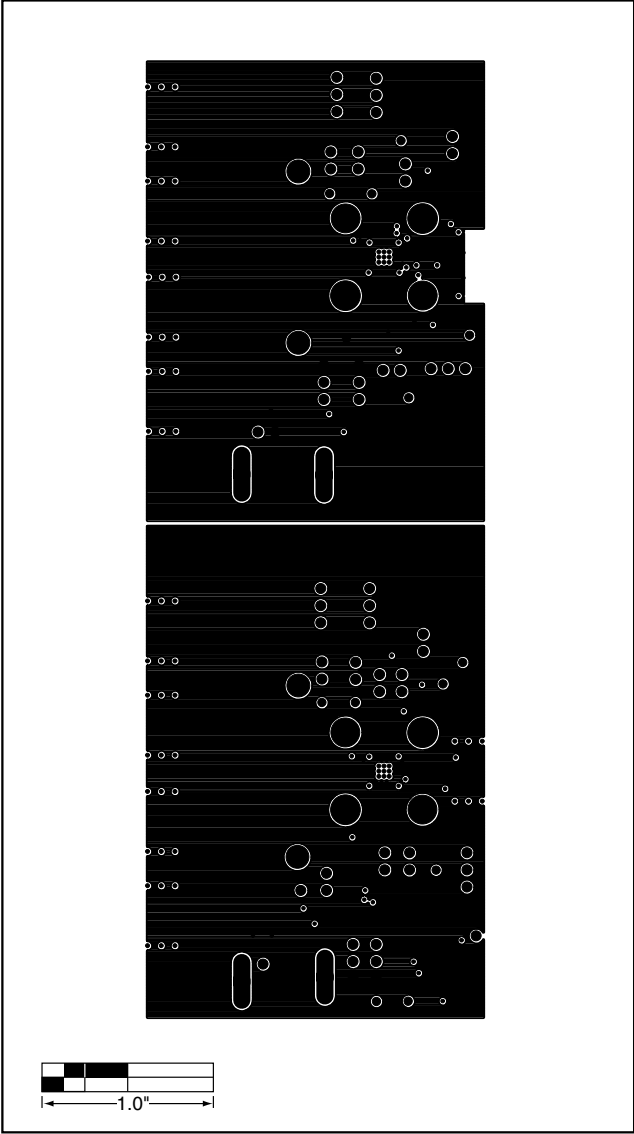
Figure 7. MAX3273 EV Kit PC Board Layout—Power Plane
